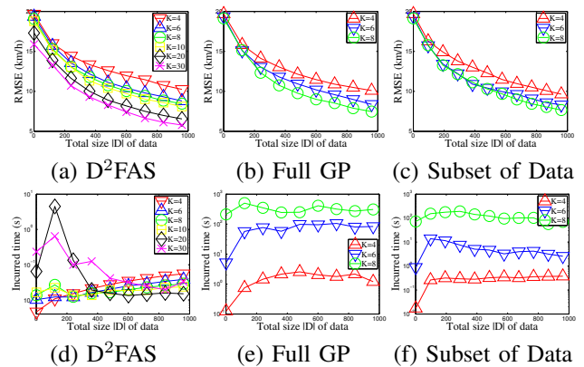
Fig. 8. Graphs of (a-c) predictive performance and (d-f) time efficiency vs. total size |D| of data gathered by varying number K of vehicles.
