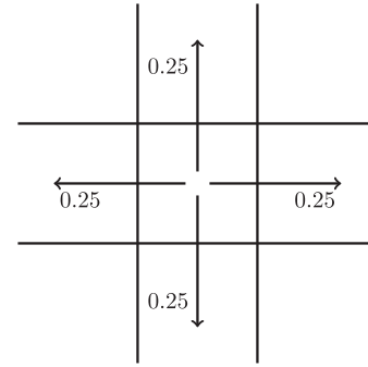
Fig. 1. Transition probabilities.
