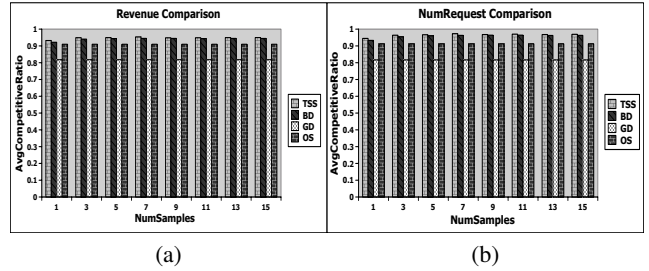
Figure 2: Dataset 1: |\mathcal{Z}| = 483 , \sum_{i \in \mathcal{Z}} N_i^1 = 2000 , \frac{1}{10} \sum_{t=1}^{10} \mathcal{D}^t = 486
